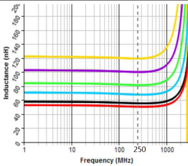
L vs Frequency
