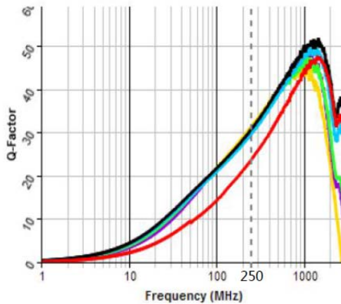
Q vs Frequency
