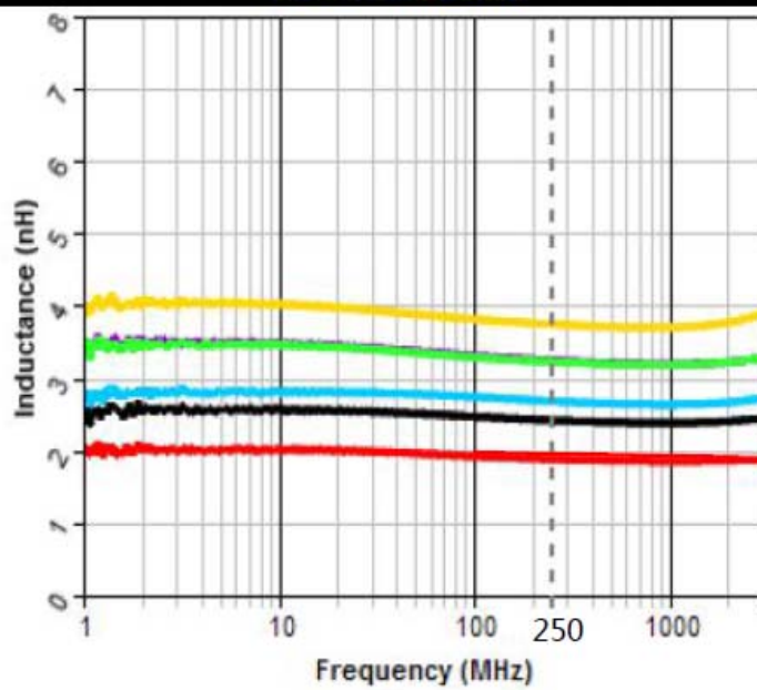
L vs Frequency
