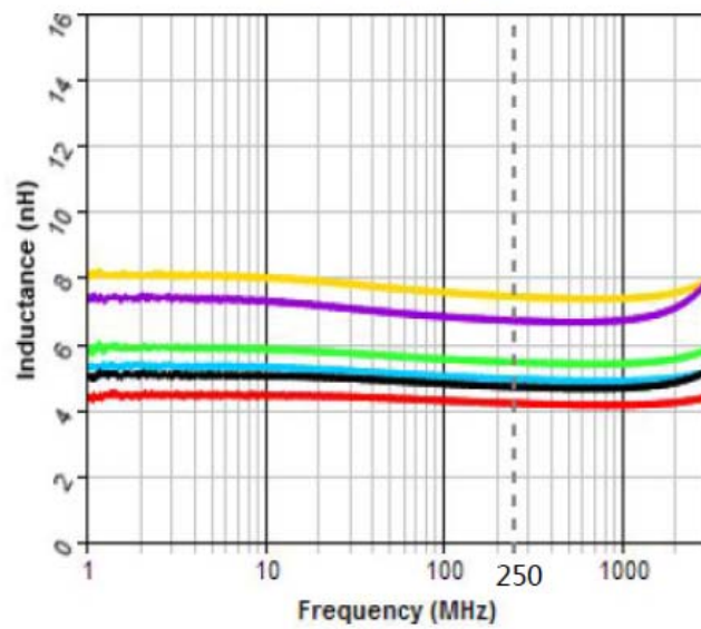
L vs Frequency
